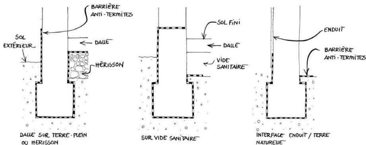
Figure 6: Barrière anti-termites
