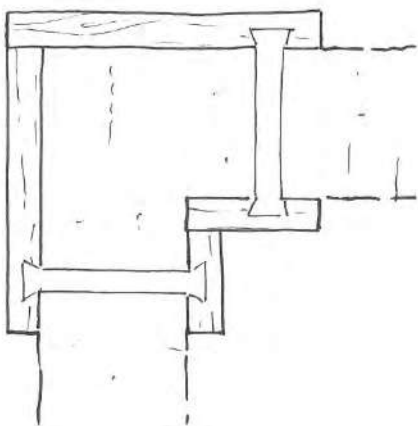
Figure 27: Agrafe* extérieure
